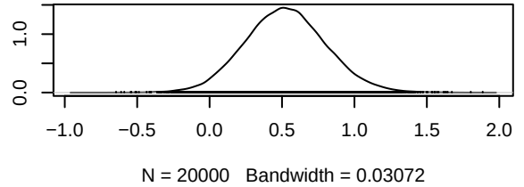
Density of d.I.III
