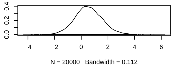
Density of d.I.Rociletinib
