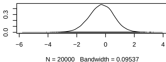
Density of d.I.DHFRi
