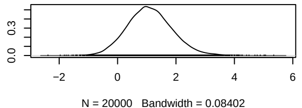
Density of d.I.Zorifertinib
